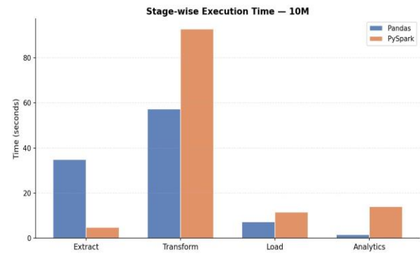
Fig. 6. Stage breakdown at 10M rows.
